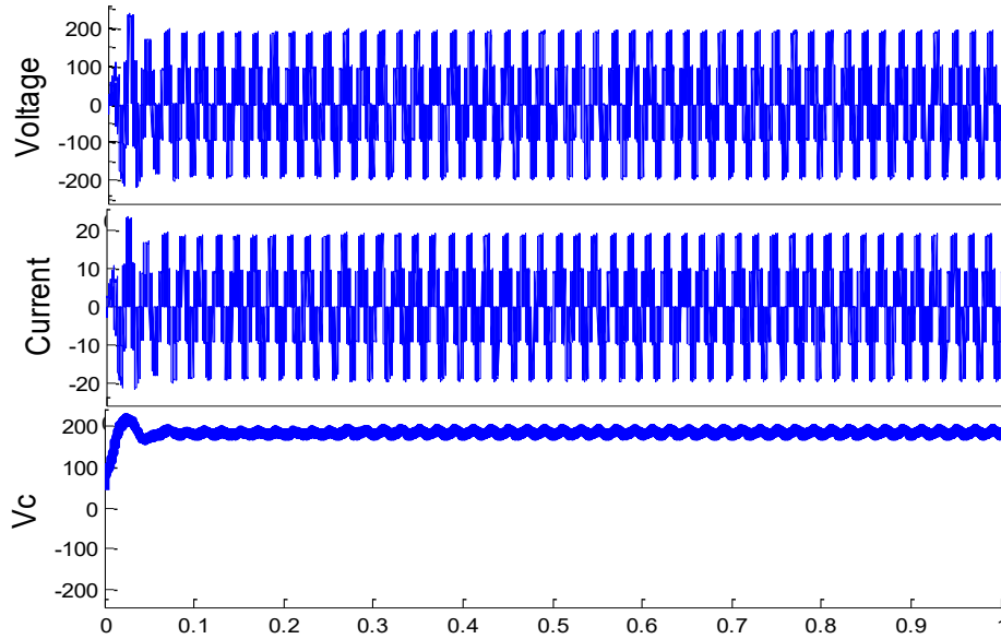
Figure 2: Output Obtained from the End Side of MCBC Scheme
