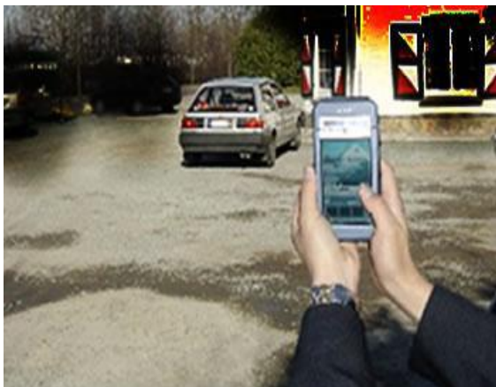
Fig 2: Take Picture
