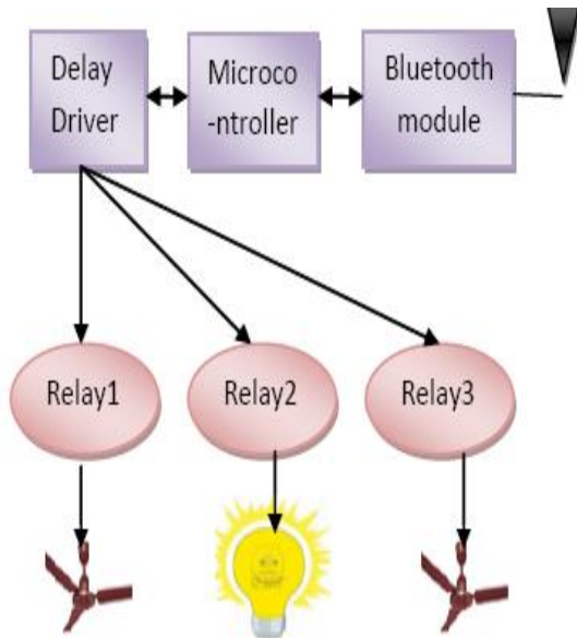
Fig 2: Block Diagram of Receiver Section
