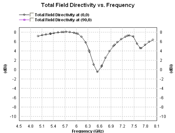
Fig 8: Total field directivity & frequency of Rectangular Micro-strip Patch Antenna with C insideC shaped slots
