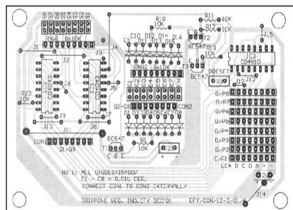
Fig 8: Component Layout
