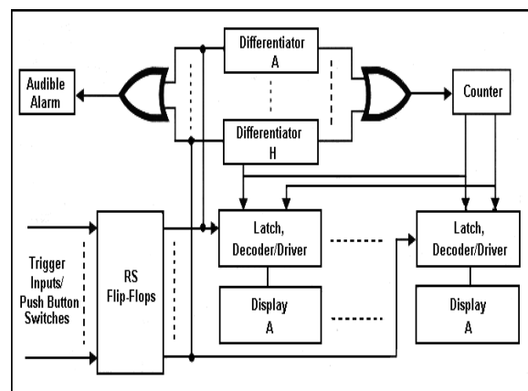
Fig: 5. Block diagram of sequential tripping
