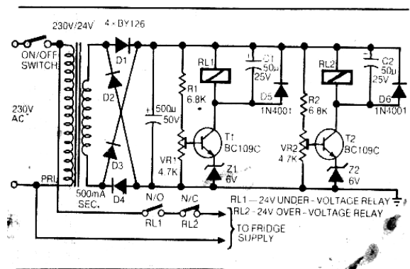
Fig 4: Circuit diagram for over/under voltage protection
