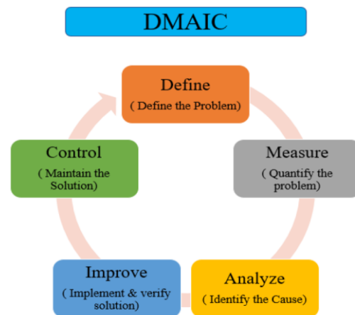
Figure 5: DMAIC Methodology [7]
