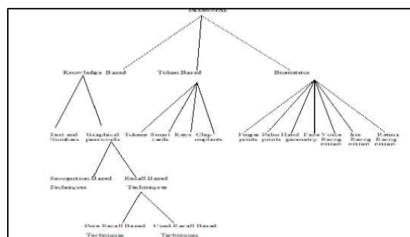
Fig 1: Authentication Methods
