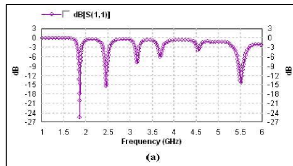
Fig 2: Return Loss of Patch Antennas (a) Base Shape (b) Single Slotted Shape (c) Five Slotted Shape
