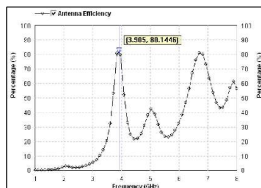
Fig 8: Radiation Efficiency Vs Frequency Curve
