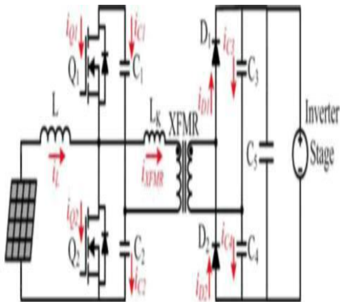
Fig 3: IBR Converter
