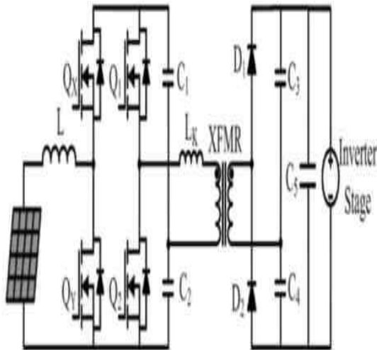
Fig 3: IBR Converter
