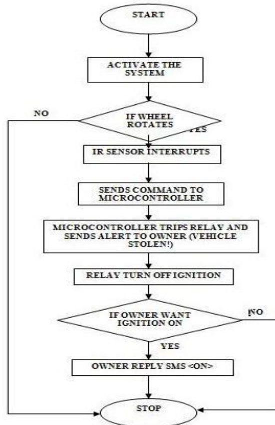
Fig 6: Flowchart for Antitheft System
