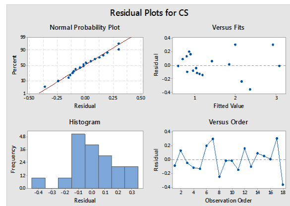
Fig. 4. Residual Plots for Cutting Speed
