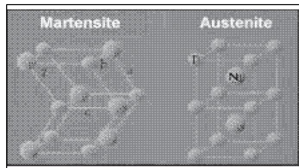
Fig 3: Microscopic and Macroscopic Views of the Two Phases of Shape Memory Alloys
