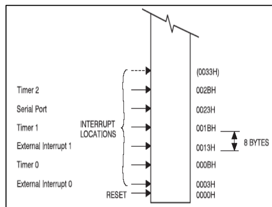
Fig. 3: Program Memory
