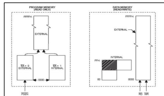
Fig. 3: Program Memory
