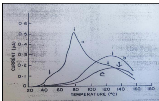
Fig 6: Open –Circuit TSC of BOPP Corona Charged to Initial Surface Potentials of -400,-800,-1000 & -1200v (curve a, b, c & d respectively) at Room Temperature.
