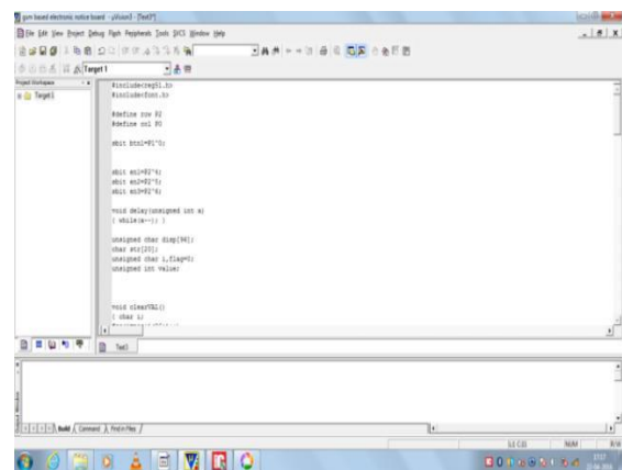
Fig 11: KEIL Software
