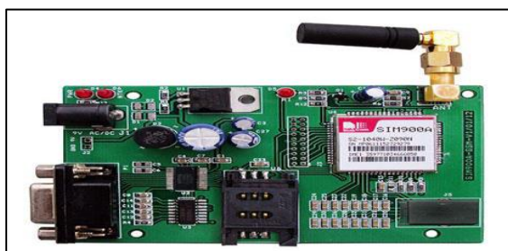
Fig 2: GSM Modem
