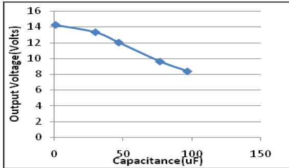
Fig 7: Output Current Versus Capacitance
