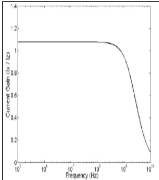
Fig 2: Frequency Response of Current Gain of CMOS CCCII Design with Basic Circuit Configuration
