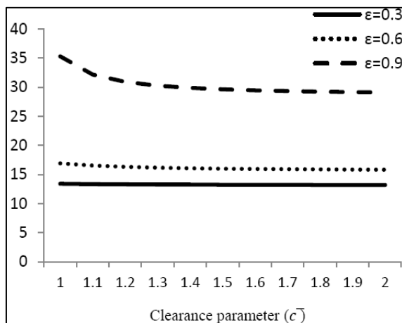
Fig. 9 Coefficient of Friction Verses Clearance at Different Eccentricity Ratio
