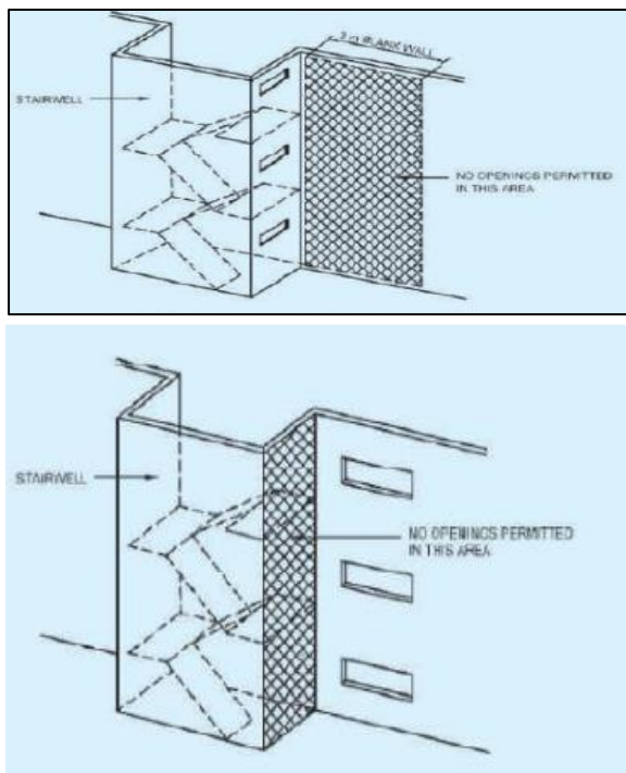
Fig. 2: Stairwalls Opening
