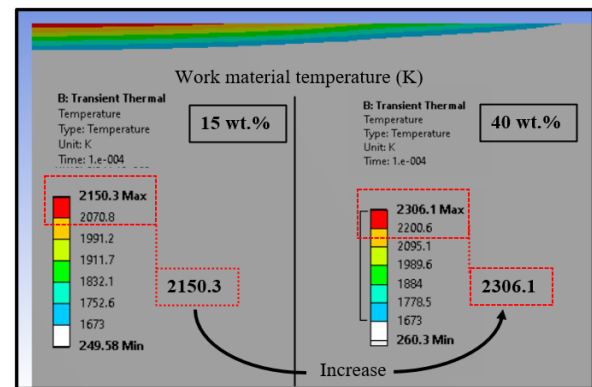
Fig. 9: Work Material Temperature Comparison at 15 wt.% and 40 wt.%
