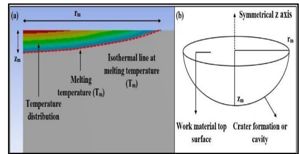
Fig. 4: Criteria of MRR Estimation [13]
