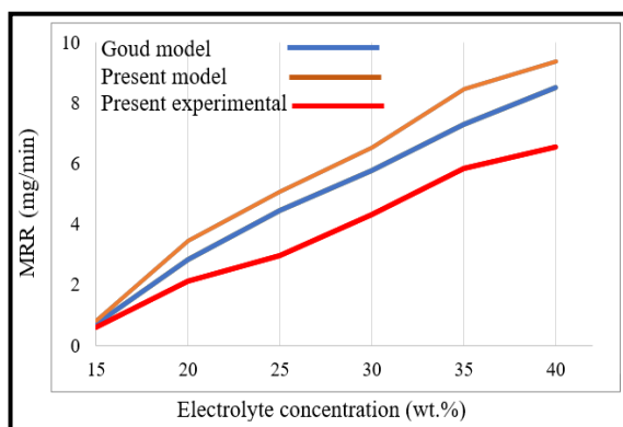
Fig. 8: Comparison of MRR Variation
