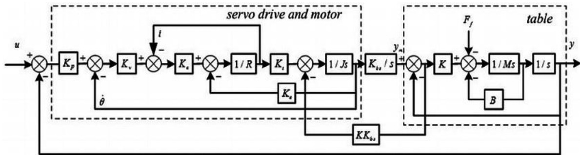
Figure 1: Feed Servo System
