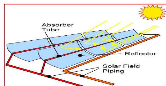
Fig 2: Solar Collector
