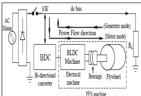
Fig 1: Typical FES System and Sources of Losses Higher Power Density
