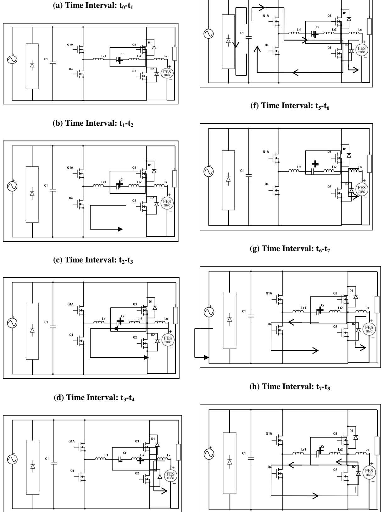
Fig 6: Current Path in the Circuit and Device Status in Boost Mode.
