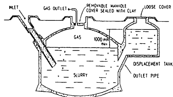
Fig 2: Schematic Diagram of a KVIC Biogas Plant
