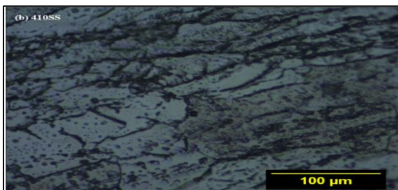
(b) Martensitic 410
