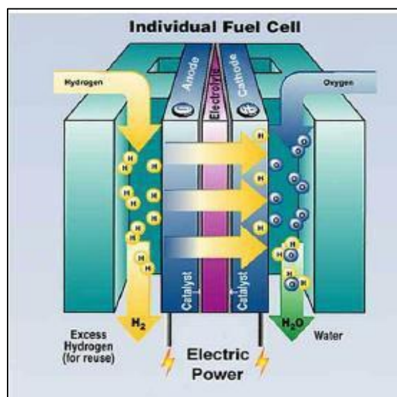
Fig 7: Working Principle of PEMF
