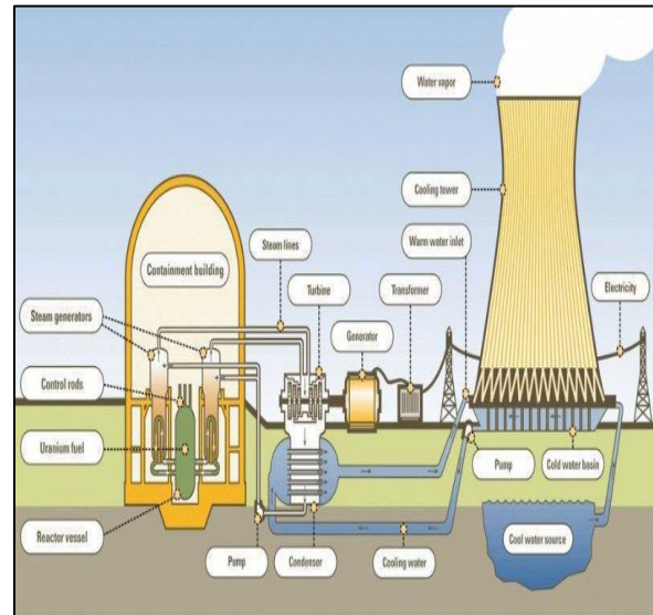
Fig 14: Block Diagram of Nuclear Power Plant
