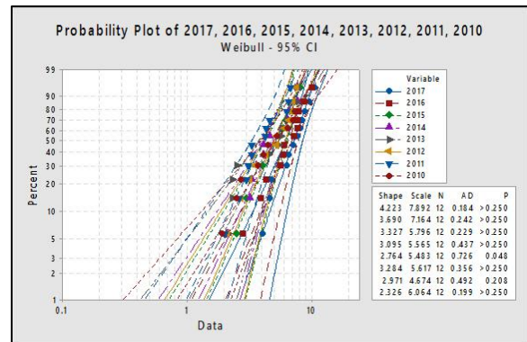
Fig 8 (b): Probability Distribution Plot for Dibrugarh City
