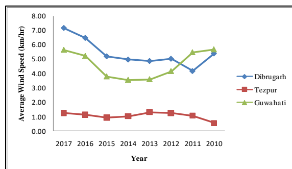
Fig.5 Variation of Wind Speed with Years from 2010-2017
