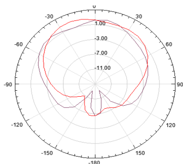
Figure 11: Radiation Pattern at 3.17GHZ
