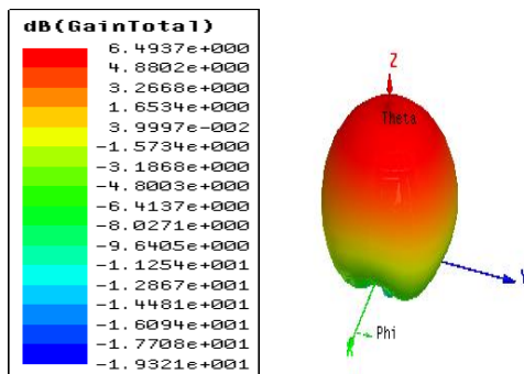
Figure 9: Radiation Pattern at 3.11GHZ
