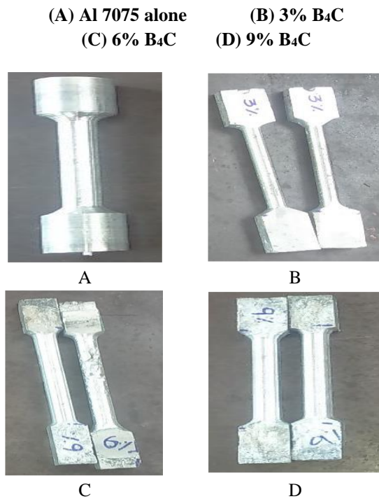
Figure 2: Fabricated Al- B_4C Composite Samples
