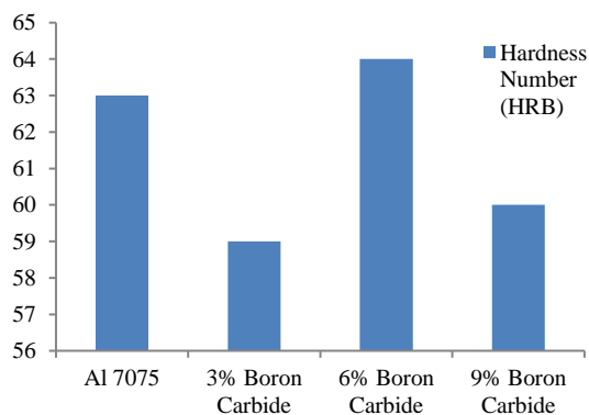
Figure 3: Variation in the Hardness of the Composite Samples
