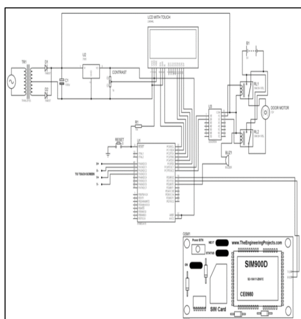
Fig 2: Circuit Diagram
