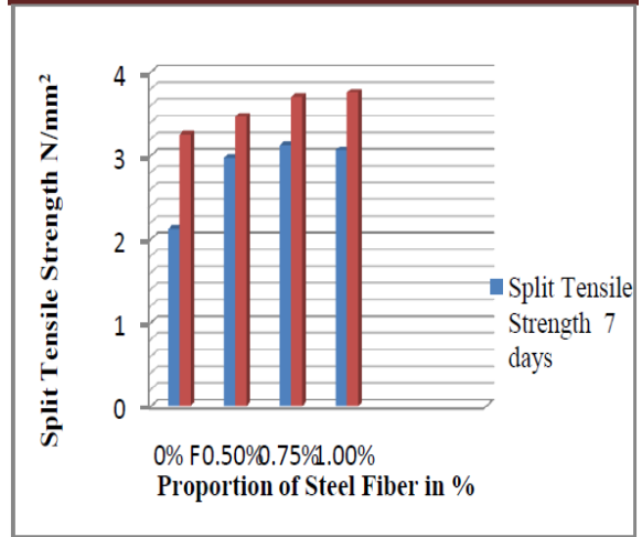
Fig 12: Split Tensile Strength of Steel Fiber After 7th and 28th Days Inference
