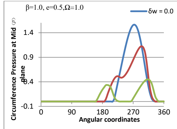
Fig 5: Circumference Pressure
