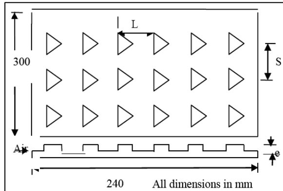
Fig 15: Type of Roughness Geometry Investigated by Bhaskar Et. Al (2011).
