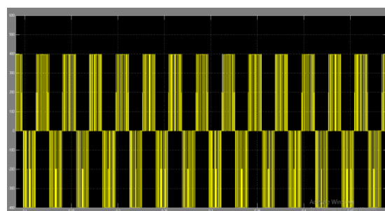
Fig 5: Waveform of Line Voltage V_{ab} for m_a=0.7
