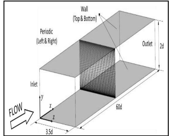
Fig 1: Schematics of computational channel domain
